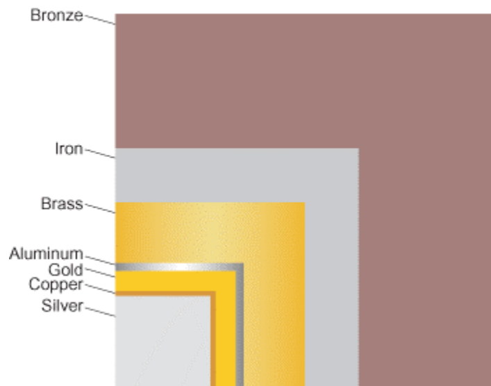
Required Material Sizes For Equivalent Conductivity
